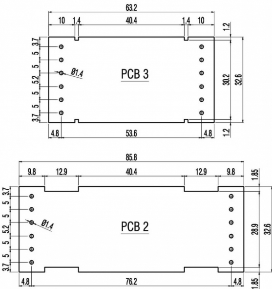
PC BOARD LAYOUT - sp. 1mm DIMENSIONI CIRCUITO STAMPATO - sp. 1mm
