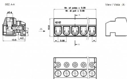
SHSxx-5,08-L
