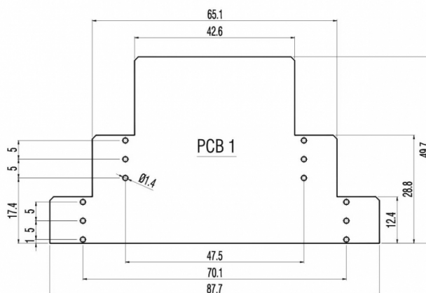
PC BOARD LAYOUT - sp. 1mm DIMENSIONI CIRCUITO STAMPATO - sp. 1mm
